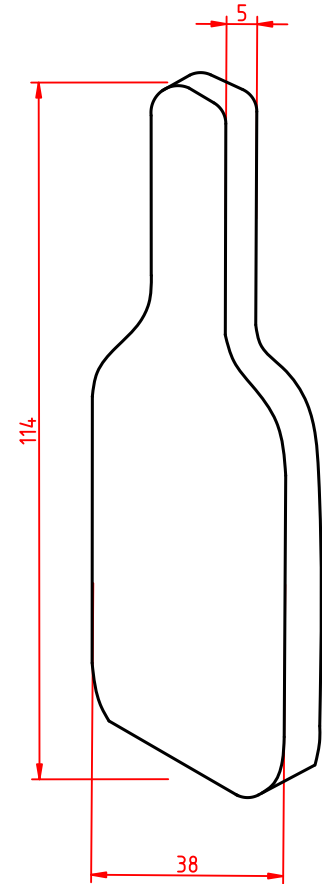
INTERIOR DIMENSIONS
